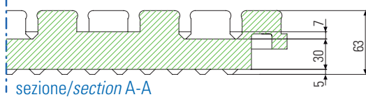
Pannello / Panels 1100 x 600 H 30
