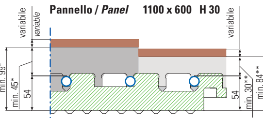
Modello H = 10 / Model H = 10
