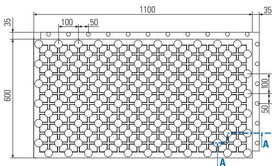
Modello H = 50 / Model H = 50
