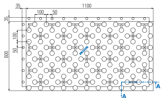
Modelli H = 20/30 / Model H = 20/30
