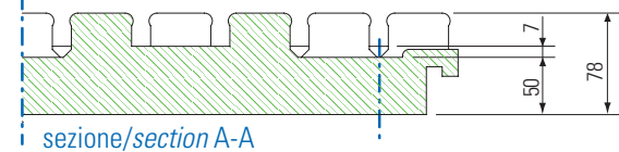
Pannello / Panels 1100 x 600 H 50
